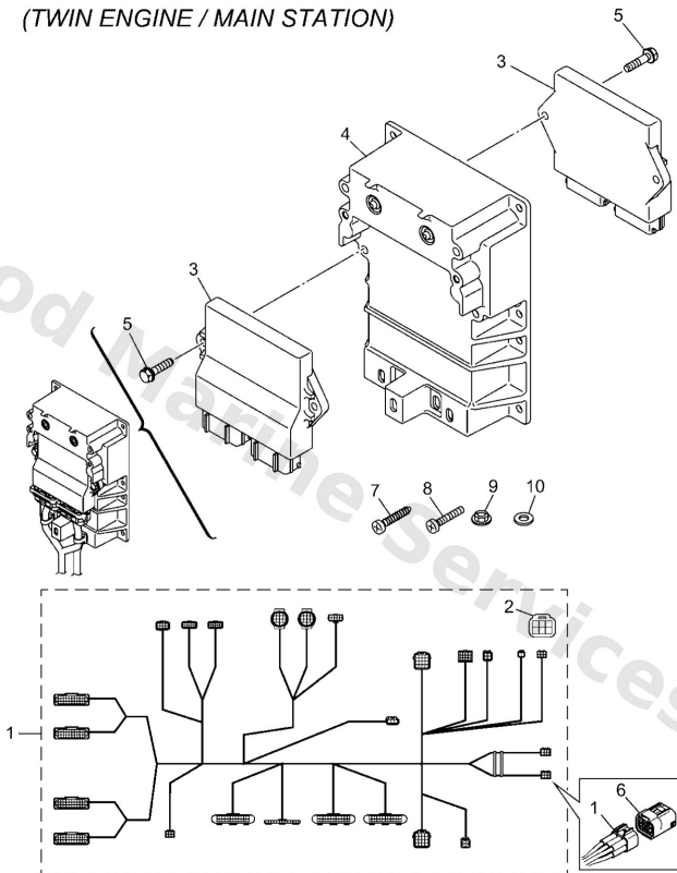
DIGITAL ELECTRONIC CONTROL (TWIN ENGINE / MAIN STATION)
