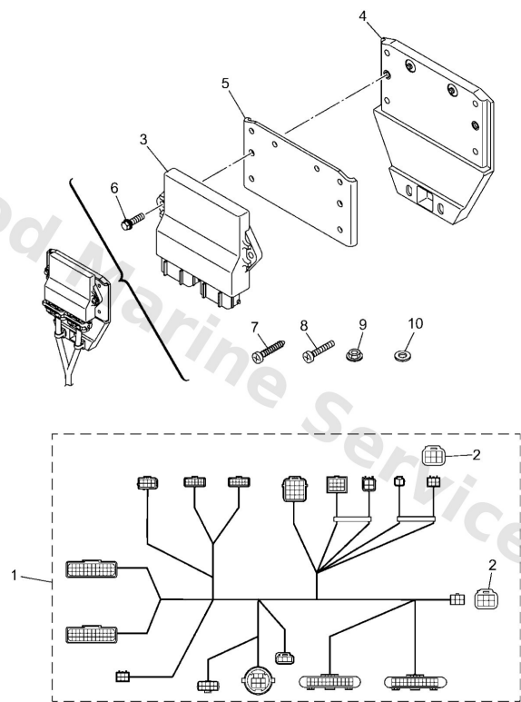
DIGITAL ELECTRONIC CONTROL (SINGLE ENGINE / MAIN STATION)
