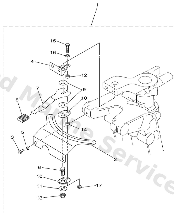
6X4 TILLER HANDLE FITTING KIT STEERING FRICTION (F30-FI / F40-FI)
