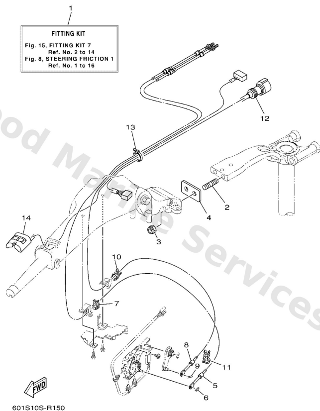
6X4 TILLER HANDLE FITTING KIT (F75B,F80D,F90B,F100F)
