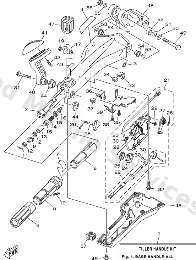
6X4 TILLER HANDLE KIT (F20F-F130A)
