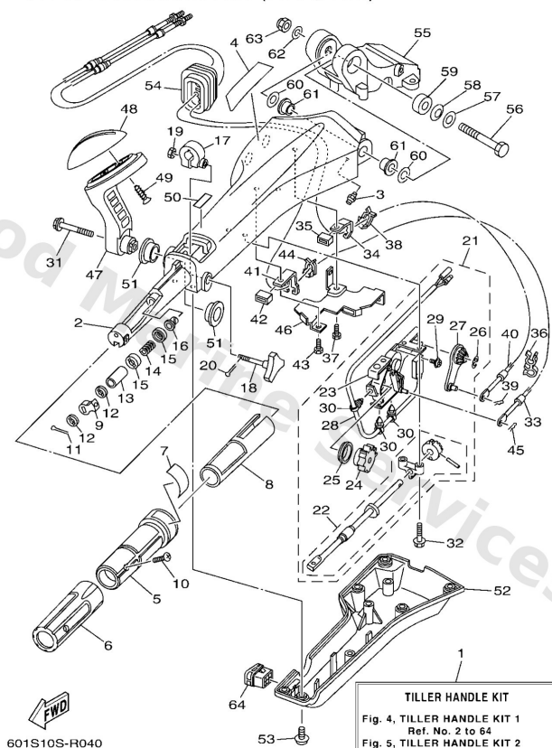
6X4 TILLER HANDLE KIT (F25A,F25B)
