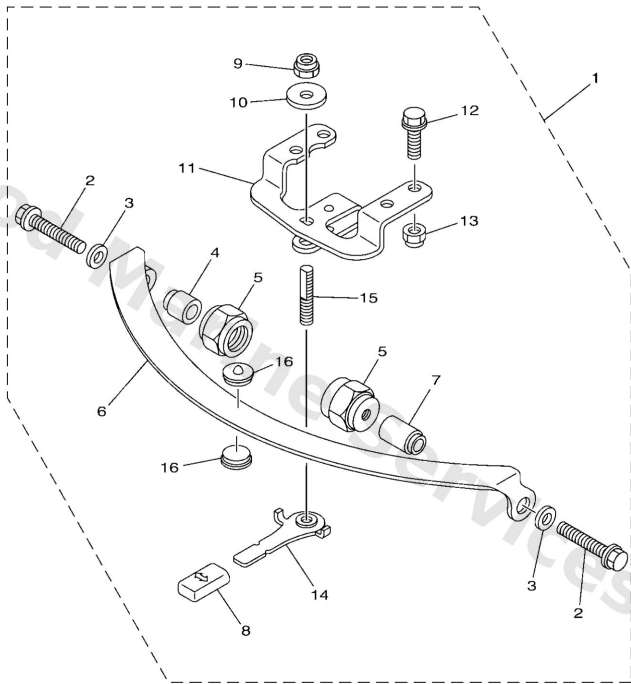
6X4 TILLER HANDLE FITTING KIT STEERING FRICTION (F75A,F75B,F80D,F90A,F90B,F100F, F115A,F115B,VF115A,F130A)
