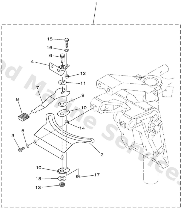
6X4 TILLER HANDLE FITTING KIT STEERING FRICTION (F50B,F50H,T50B,FT50J, F60B,F60F,T60B,FT60G,F70A)
