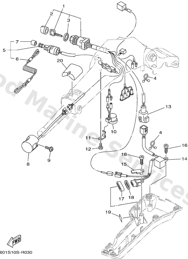
6X4 TILLER HANDLE KIT (F20F-F130A FOR EU&ANZ)
