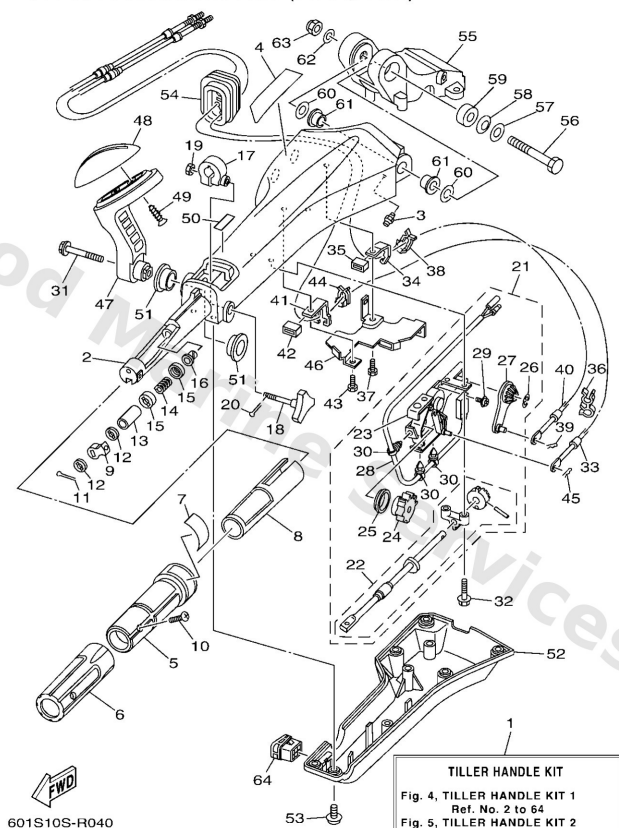
6X4 TILLER HANDLE KIT (F25A,F25B)
