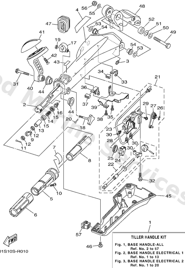
6X4 TILLER HANDLE KIT (F20F-F130A)
