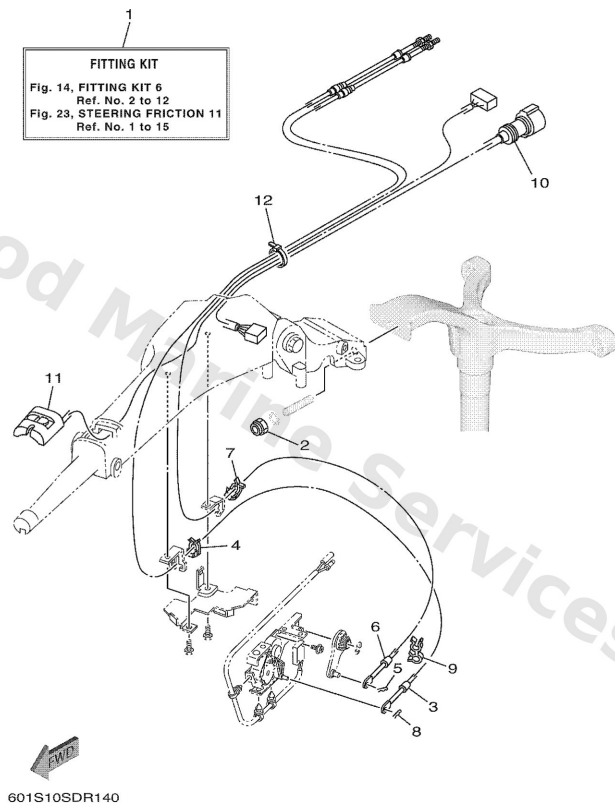
6X4 TILLER HANDLE FITTING KIT (F20F,F25C,F25G)
