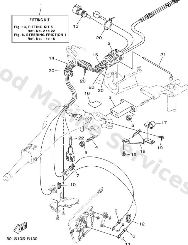
6X4 TILLER HANDLE FITTING KIT (F115A)
