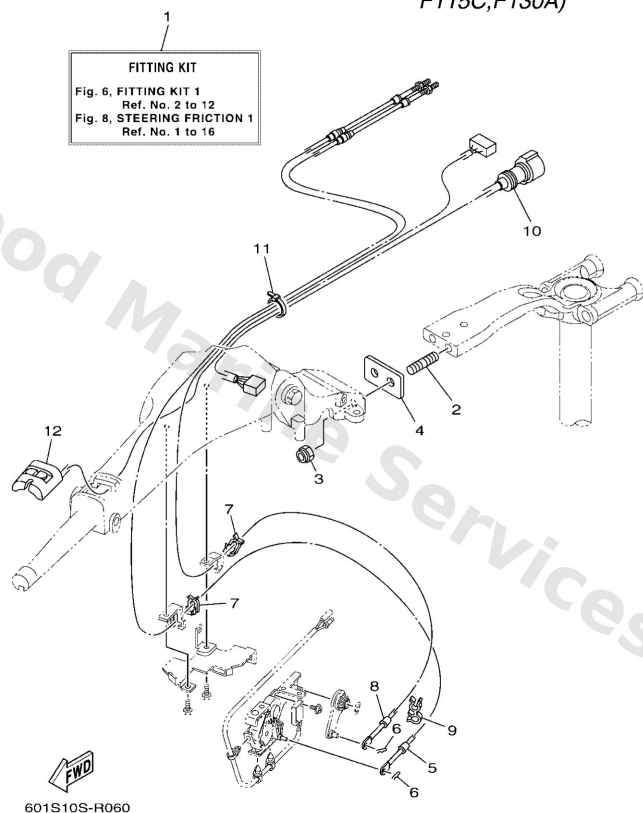
6X4 TILLER HANDLE FITTING KIT (F115B,VF115A, F115C,F130A)
