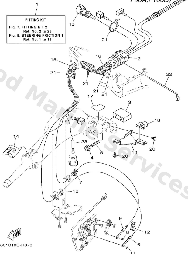
6X4 TILLER HANDLE FITTING KIT (F75A,F75B,F80D, F90A,F100D)
