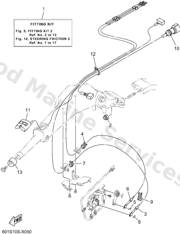
6X4 TILLER HANDLE FITTING KIT (F50B,F50H,T50B,FT50J,F60B,F60F,T60B,FT60G,F70A)
