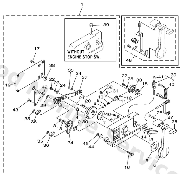
701 REMOTE CONTROL (PULL TO OPEN TYPE)
