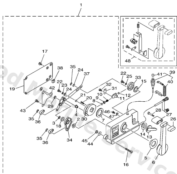
701 REMOTE CONTROL (PUSH TO OPEN TYPE)
