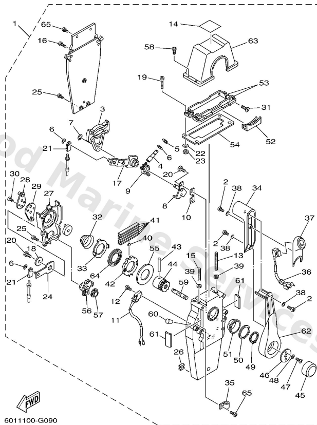
704 REMOTE CONTROL (STANDARD SINGLE)
