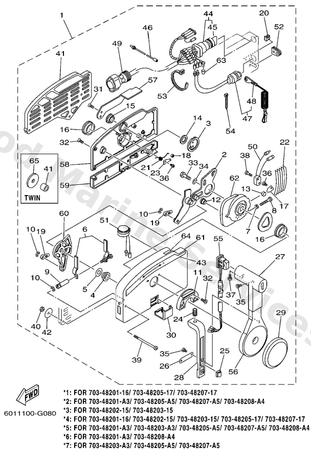
703 REMOTE CONTROL (PUSH TO OPEN TYPE)
