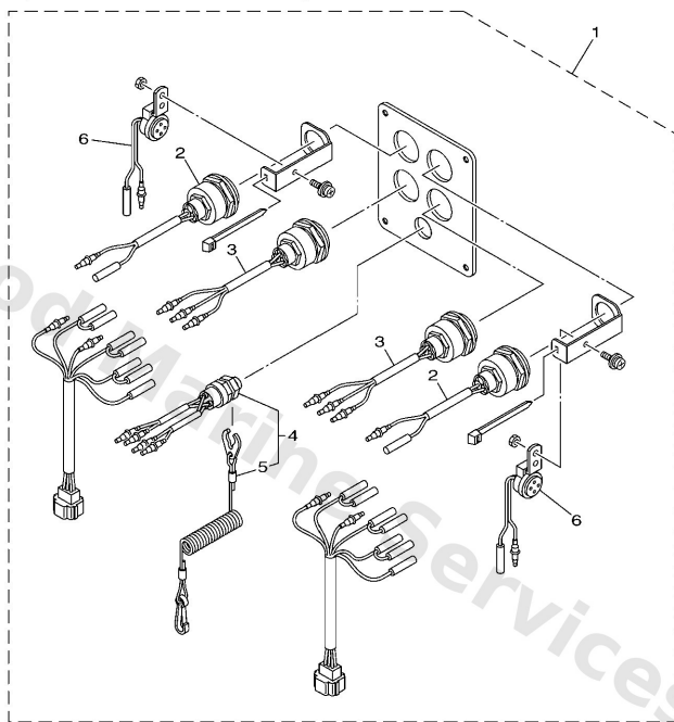
TWIN KEY SWITCH (FOR DBW REMOTE CONTROL)
