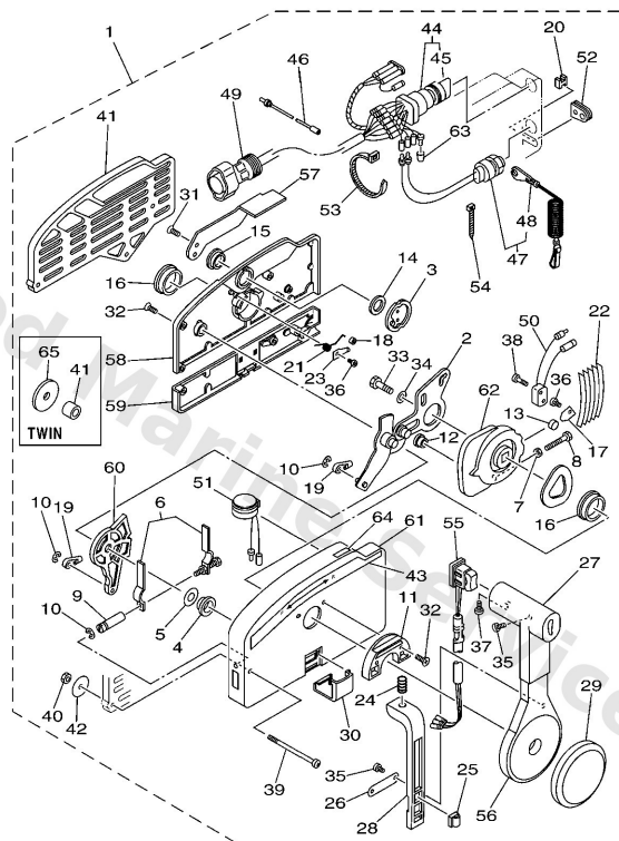
703 REMOTE CONTROL (PUSH TO OPEN TYPE)
