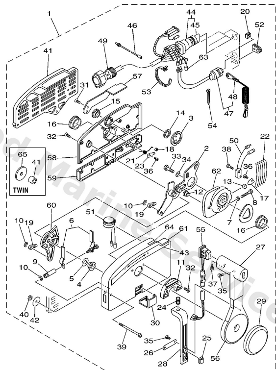
703 REMOTE CONTROL (PUSH TO OPEN TYPE)
