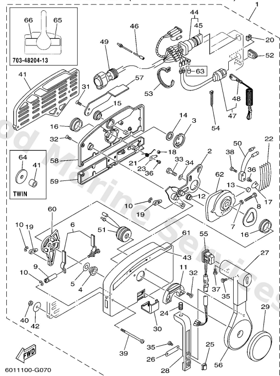
703 REMOTE CONTROL (PULL TO OPEN TYPE)
