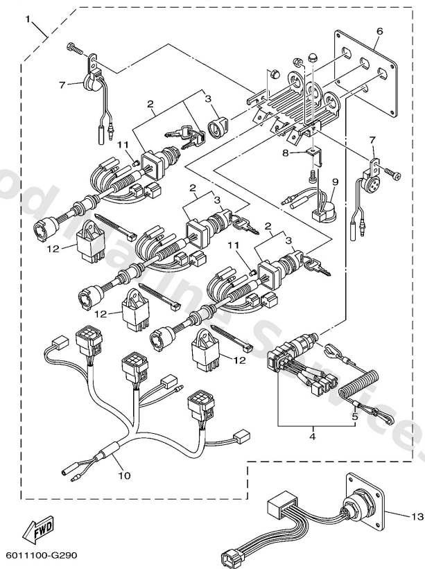
TRIPLE KEY SWITCH (FOR DIGITAL NETWORK GAUGE)
