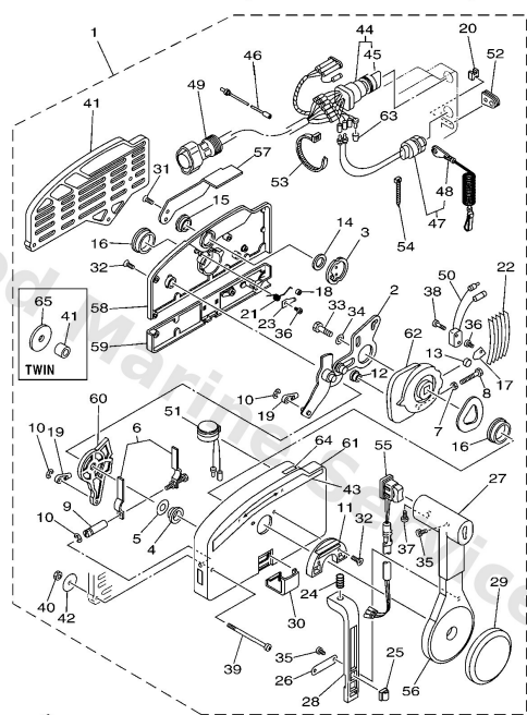
703 REMOTE CONTROL (PUSH TO OPEN TYPE)
