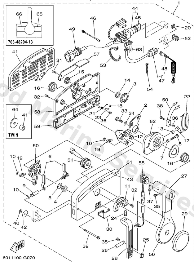
703 REMOTE CONTROL (PULL TO OPEN TYPE)
