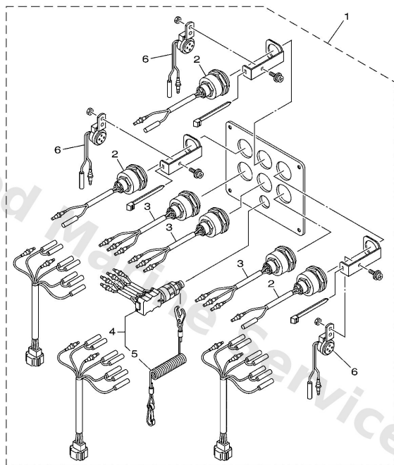
TRIPLE KEY SWITCH (FOR DBW REMOTE CONTROL)
