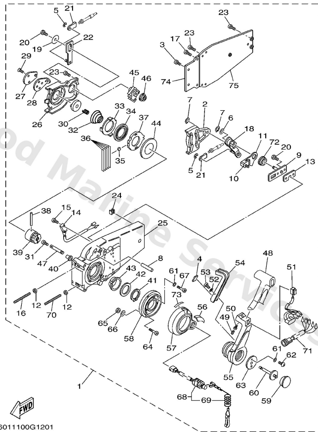
6X3 REMOTE CONTROL
