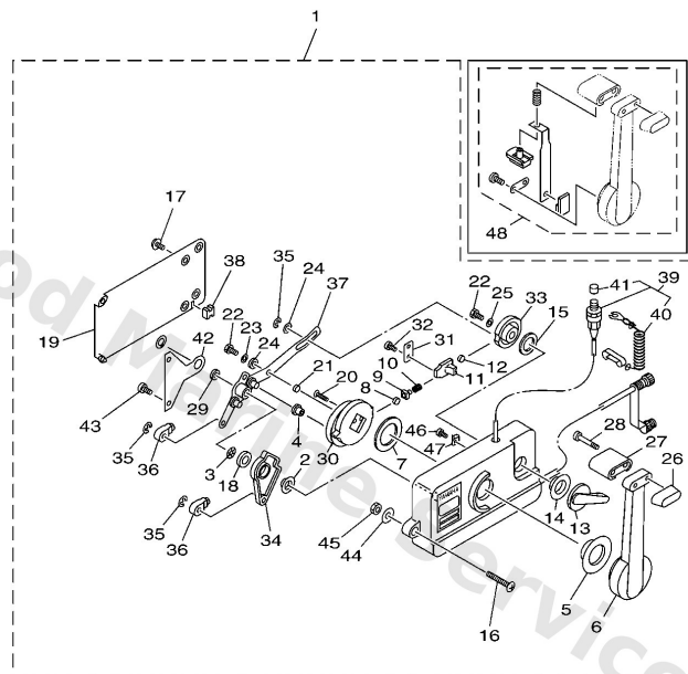
701 REMOTE CONTROL (PUSH TO OPEN TYPE)
