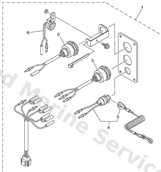
SINGLE KEY SWITCH W/ PANEL (FOR DBW REMOTE CONTROL)
