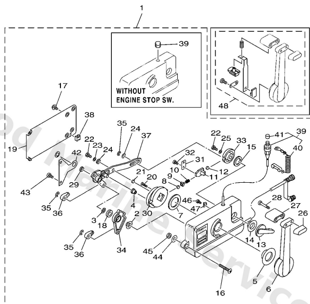
701 REMOTE CONTROL (PULL TO OPEN TYPE)
