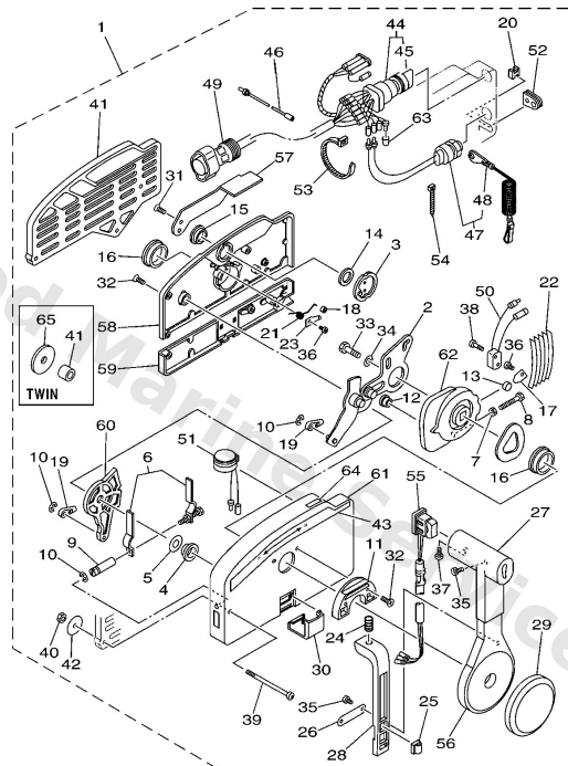
703 REMOTE CONTROL (PUSH TO OPEN TYPE)
