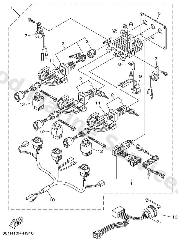
TRIPLE IG SWITCH (FOR DIGITAL NETWORK GAUGE)
