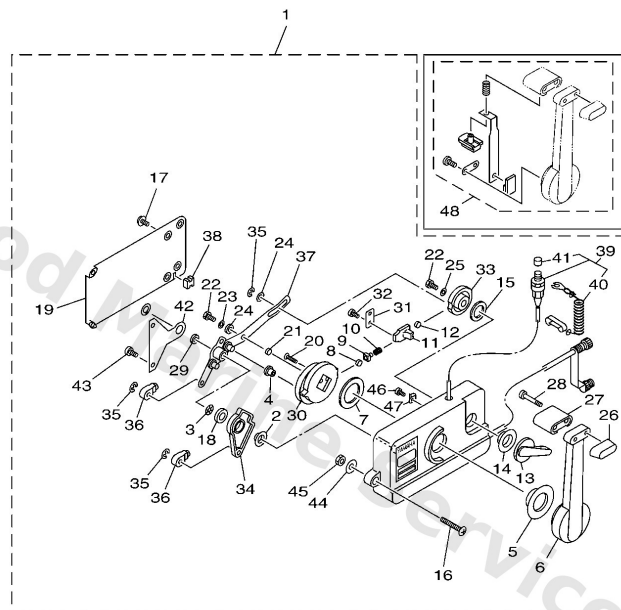
701 REMOTE CONTROL (PUSH TO OPEN TYPE)
