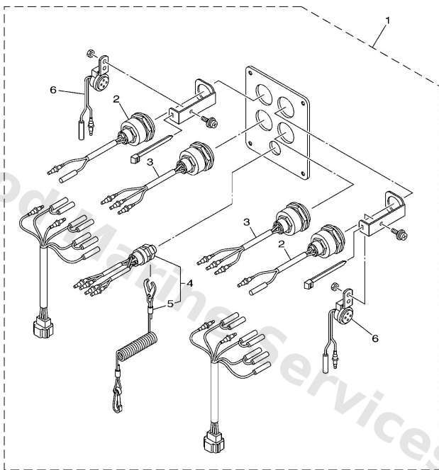
TWIN IG SWITCH (FOR 6X6 DBW REMOTE CONTROL)
