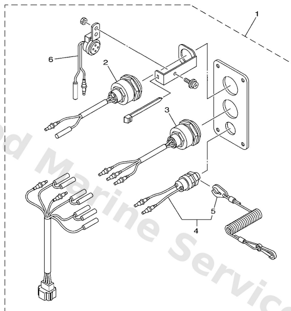
SINGLE IG SWITCH W/ PANEL (FOR 6X6 DBW REMOTE CONTROL)
