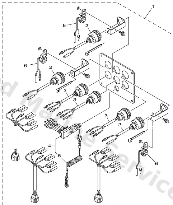
TRIPLE IG SWITCH (FOR 6X6 DBW REMOTE CONTROL)
