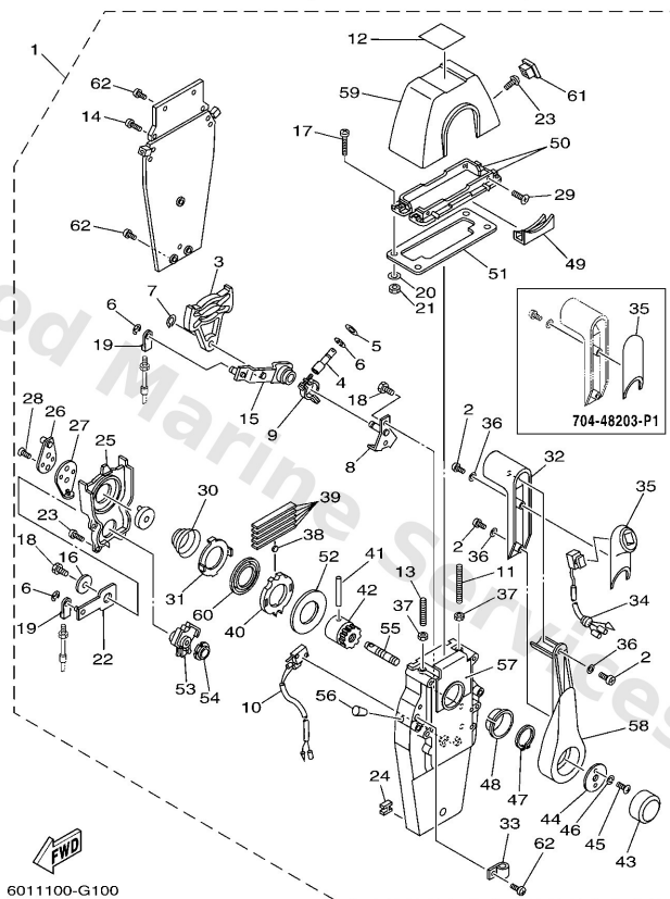
704 REMOTE CONTROL (PREMIUM SINGLE)
