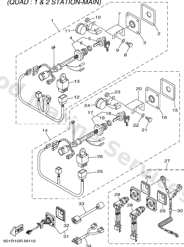
DIGITAL NETWORK SYSTEM-6Y9 (QUAD : 1 & 2 STATION-MAIN)
