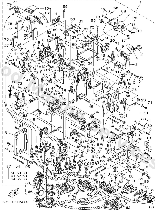
6X6 REMOTE CONTROL (TRIPLE)
