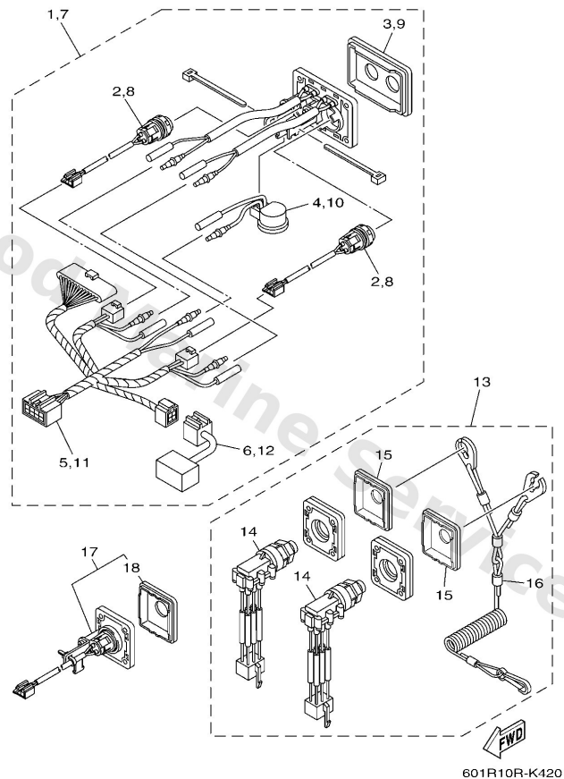
DIGITAL NETWORK SYSTEM-6Y9 (QUAD : 2 STATION-SUB)
