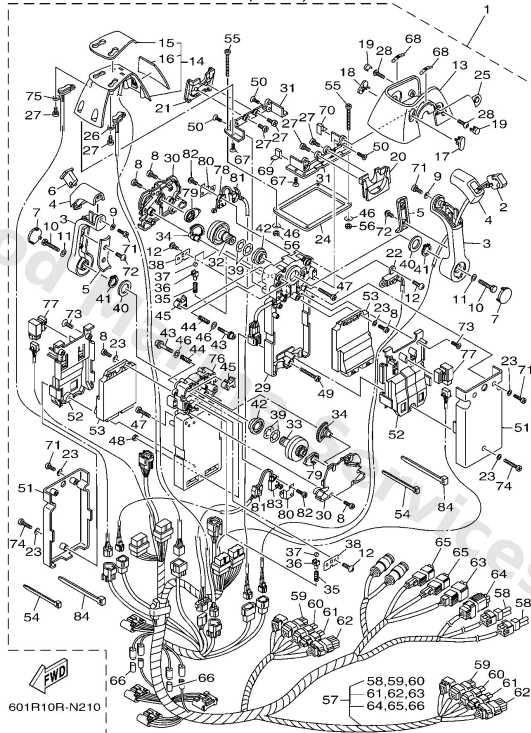
6X6 REMOTE CONTROL (TWIN)
