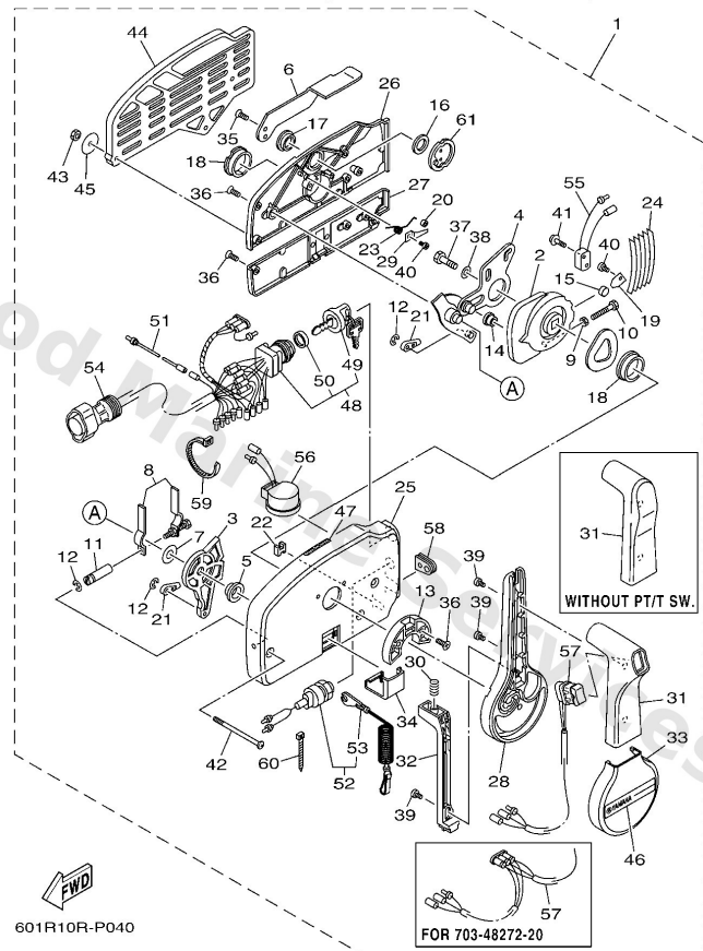
703 REMOTE CONTROL (PULL TO OPEN TYPE)
