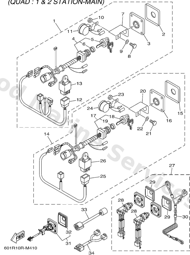
DIGITAL NETWORK SYSTEM-6Y9 (QUAD : 1 & 2 STATION-MAIN)
