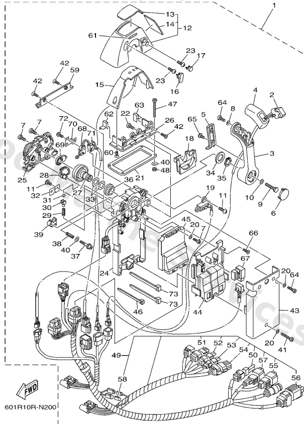
6X6 REMOTE CONTROL (SINGLE)
