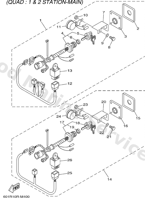
DIGITAL NETWORK SYSTEM-6Y9 (QUAD : 1 & 2 STATION-MAIN)
