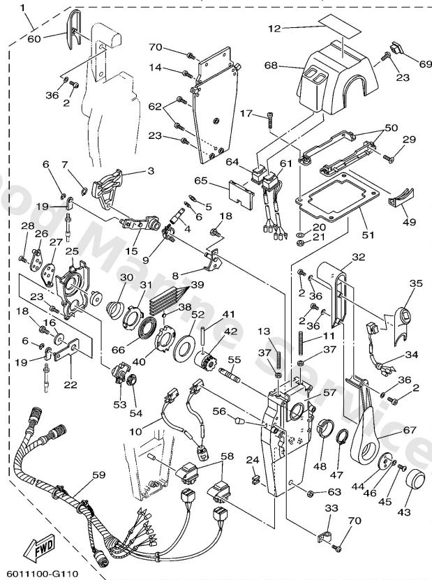
704 REMOTE CONTROL (PREMIUM TWIN)
