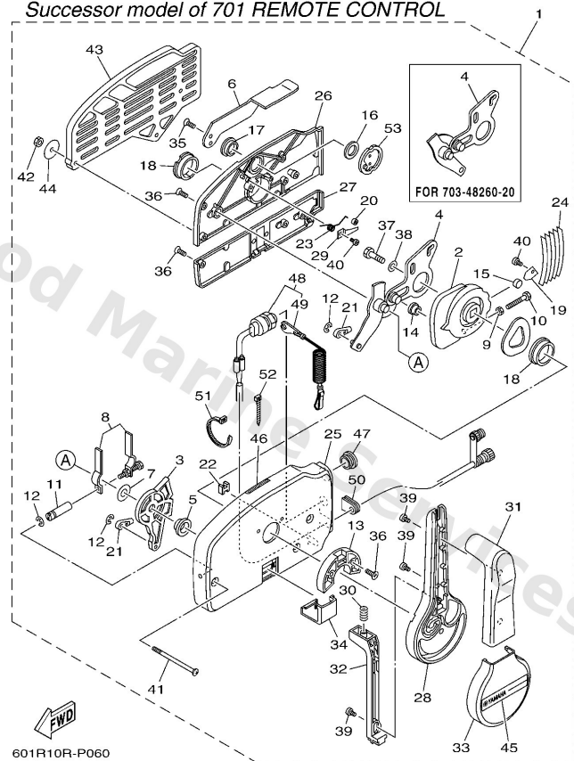
703 REMOTE CONTROL Successor model of 701 REMOTE CONTROL
