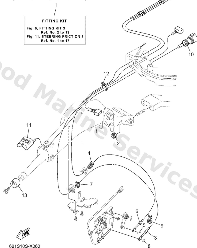
6X4 TILLER HANDLE FITTING KIT (F30A,F30B,F40A,F40F)
