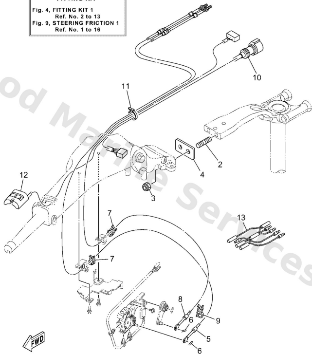
6X4 TILLER HANDLE FITTING KIT (F75B,VF90A/B,F90B, VF115A/B,F115B,F130A)
