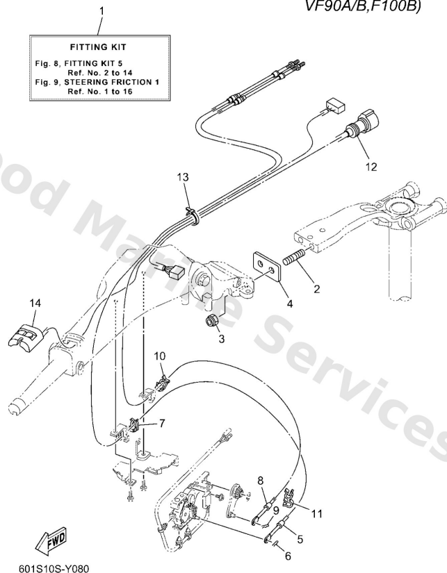
6X4 TILLER HANDLE FITTING KIT (F75B,F80B,F90B, VF90A/B,F100B)
