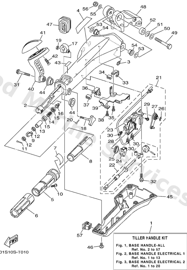
6X4 TILLER HANDLE KIT (F20B-F130A)
