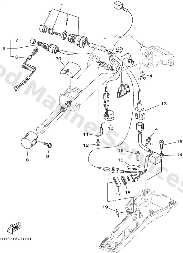
6X4 TILLER HANDLE KIT (F20G-F130A FOR EUROPE,OCEANIA)
