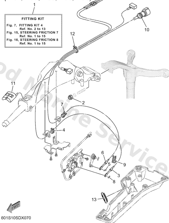
6X4 TILLER HANDLE FITTING KIT (F20B,F20G,F25C,T25C,F25G)
